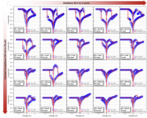
Fig. 4. Simulated I(V) loops with the extracted parameters
