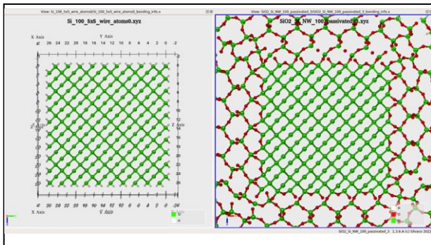
Fig. 4. Si NW [100] passivation of the dangling bonds with hydrogen atoms (left), with cristobalite \text{SiO}_2 (right).
