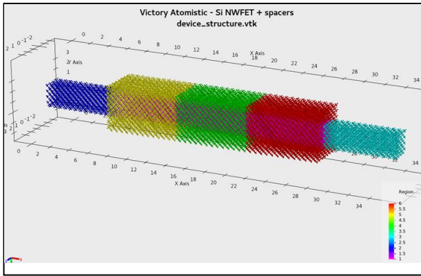
Fig. 1. MOSFET structure of a silicon nanowire oriented [100] with a square cross-section of 3 \times 3 \text{ nm}^2 .
