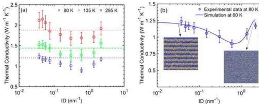
Fig. 1: (a) Experimental values of the cross-plane thermal conductivity at 80 K (blue), 135 K (green), and 295 K (red) vs interface density ranging from 0.0374 to 2.19 nm -1 . The dashed horizontal lines represent the reference values for the bulk quaternary alloys of the same stoichiometry as the SLs. (b) Experimental (open symbols) and modeling values (solid curve) for the cross-plane thermal conductivity as a function of interface at 80 K. Symbols are experimental averages, and error bars are the standard deviation of four measurements. Insets to panel (b) depict simulated structures with low and high interface densities. Reprinted with permission from AIP Publishing from Appl. Phys. Lett. 121, 232201 (2022).
