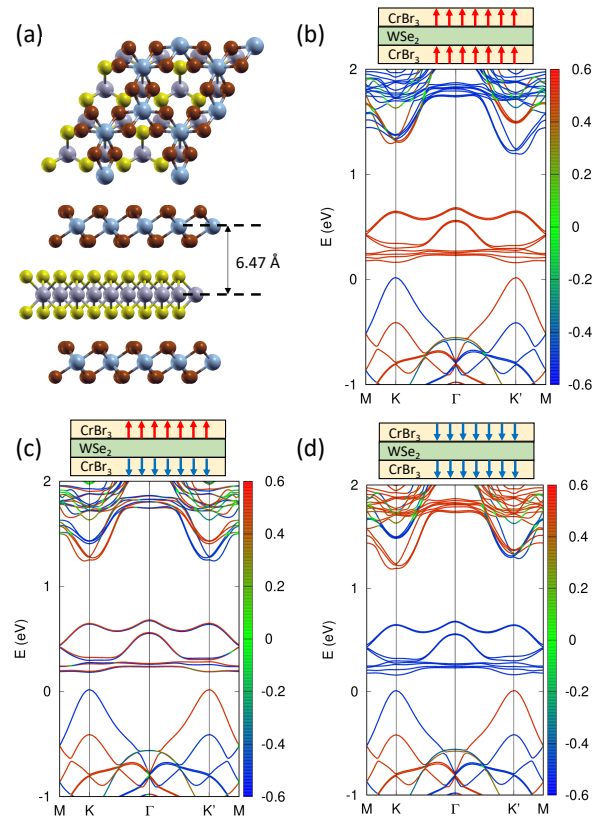
Fig. 4. (a) Details of the stacking configuration of \text{CrBr}_3/\text{WSe}_2/\text{CrBr}_3 trilayer heterostructure. Gray and yellow spheres correspond to W and Se atoms, respectively. Blue and brown spheres correspond to Cr and Br atoms, respectively. First-principles band structure for three different magnetic orientations: (b) \text{CrBr}_3 layers are co-polarized up, (c) \text{CrBr}_3 layers are counter-polarized, and (d) \text{CrBr}_3 layers are co-polarized down. Insets illustrate the magnetic configurations of the \text{CrBr}_3 layers in each case.
